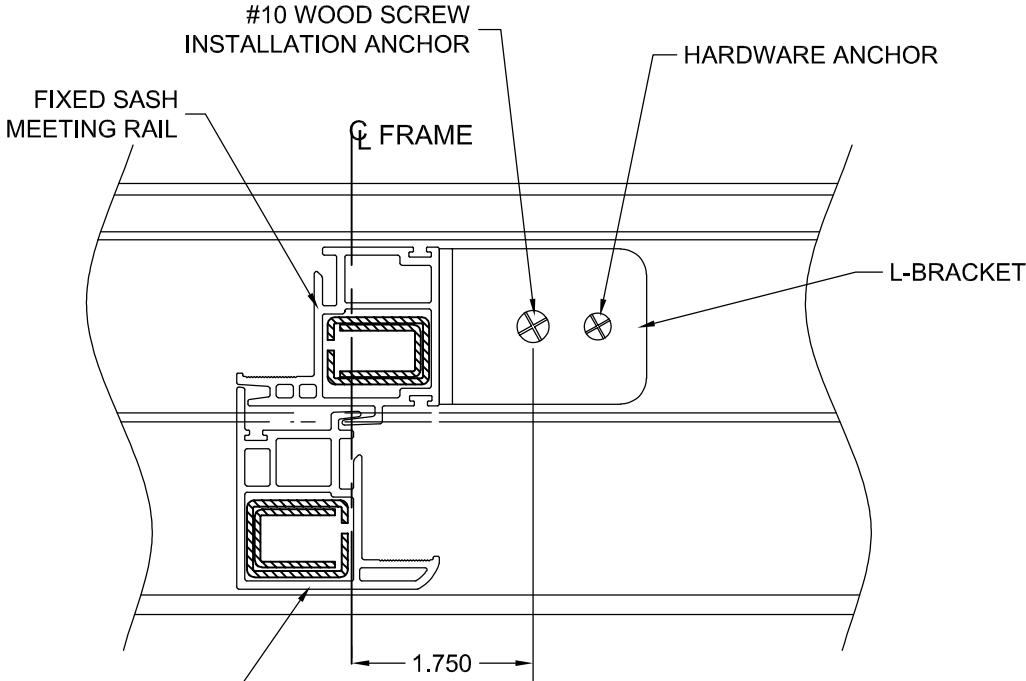
SECTION A-A L-BRACKET DETAIL IN HEAD
