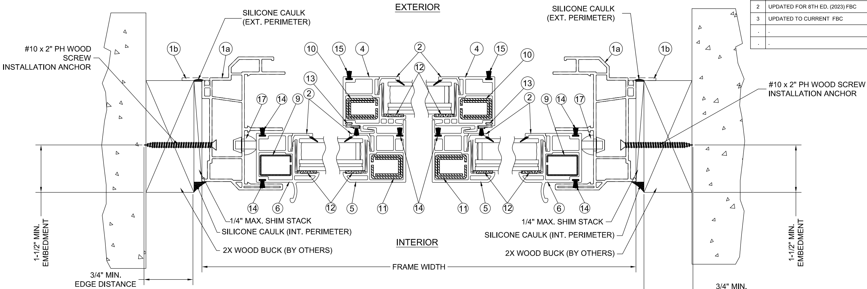
1 HORIZONTAL CROSS SECTION (2X BUCK) 07-09 RETRO / 07-10 FLANGE INSTALLATION
