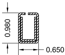
10 ST-336/ST-339 KEEPER STILE REINFORCEMENT 0.060 GALV. STEEL
