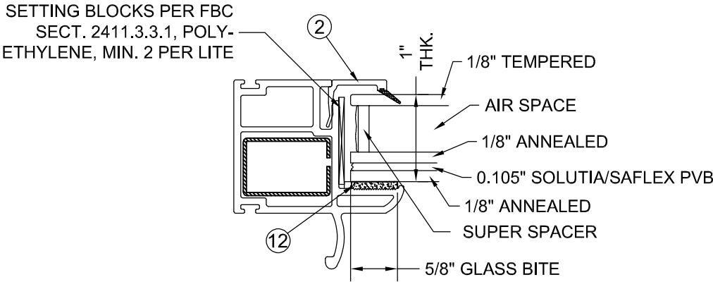
GLAZING DETAIL WITH SOLUTIA/SAFLEX LAMINATE
