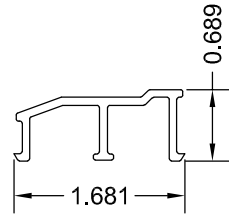
7 V355 TRACK INSERT 0.079" WALL THK.
