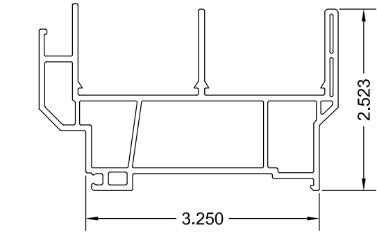
1a SL0901S HORIZONTAL ROLLER FRAME 0.079" EXT. WALL THK. 0.060" INT. WALL THK.
