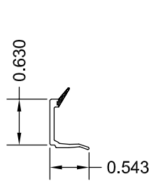
2 BV18 GLAZING BEAD 0.059" WALL THK.
